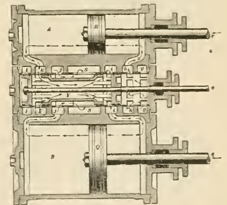
FIG. 5. PISTON VALVE USED IN VAUCLAIN COMPOUND.
